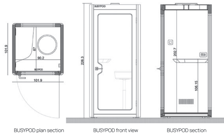
BUSYPOD plan section
